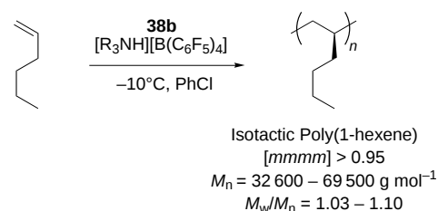
Scheme 21. Living isospecific polymerization of 1-hexene with zirconium amidinate catalysts.
